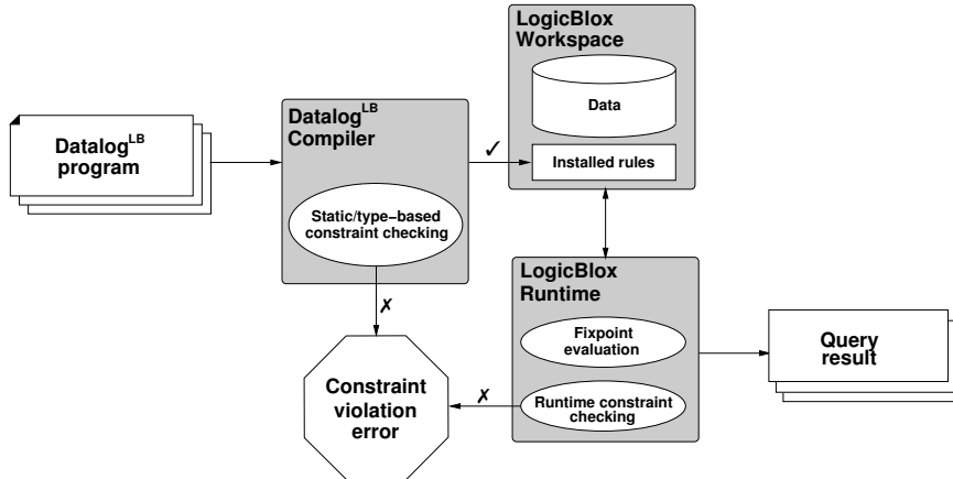
Fig. 2: LogicBlox Architecture
