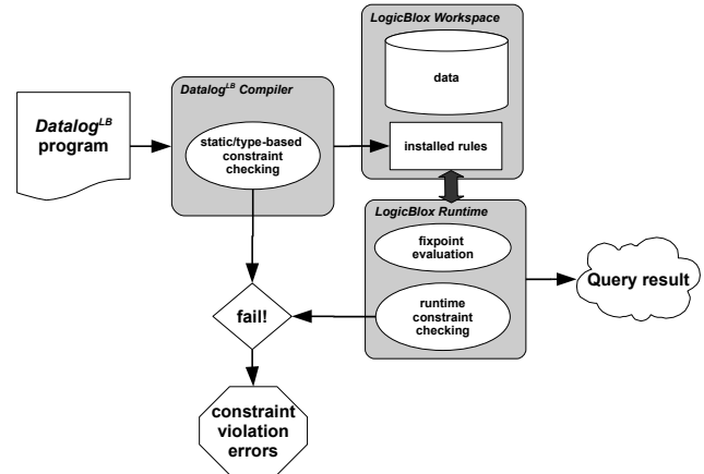
Figure 1: LogicBlox Architecture
