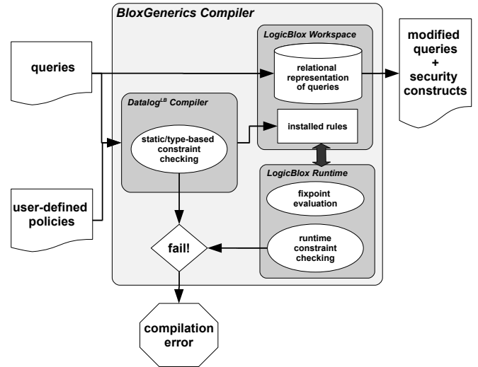
Figure 3: Detailed View of BloxGenerics Compiler
